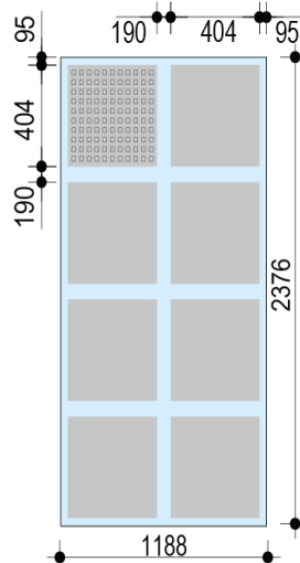
Standard Square Type B8 - 8/18Q
