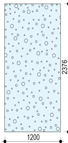
Random PLUS 12/20/35 R
